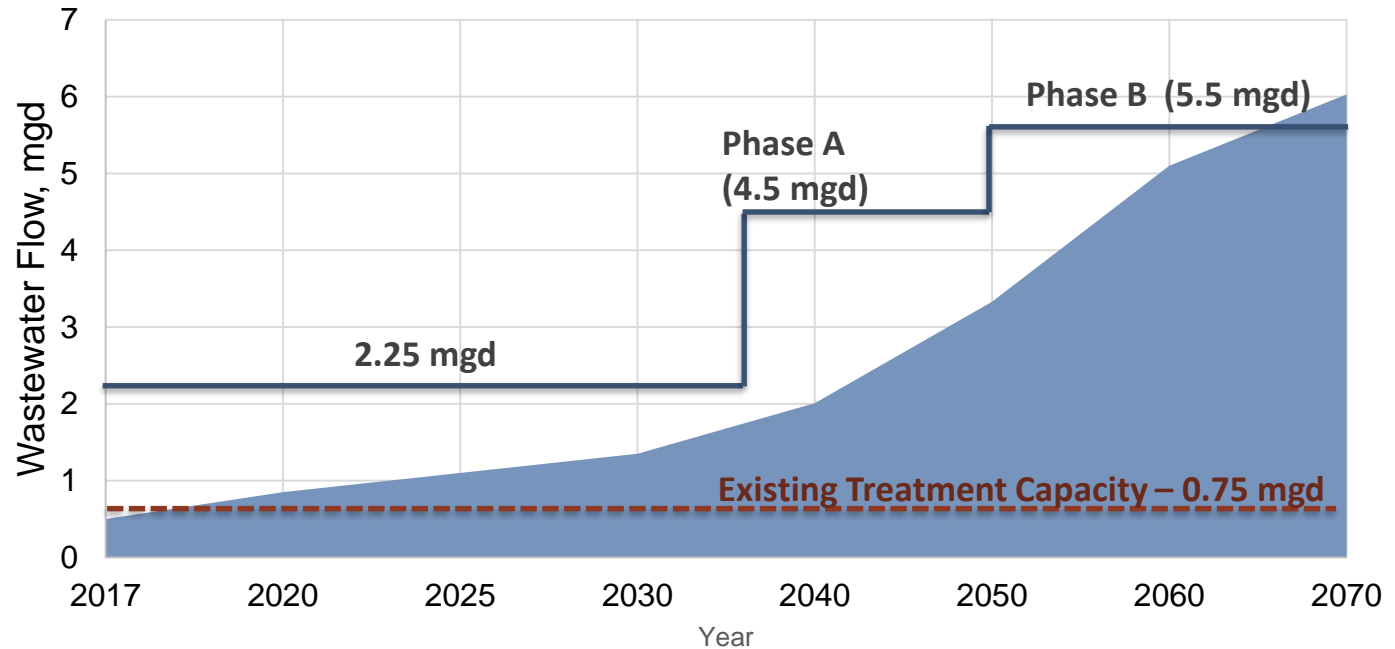
Pittsboro - Wastewater Flow vs. Treatment Capacity
