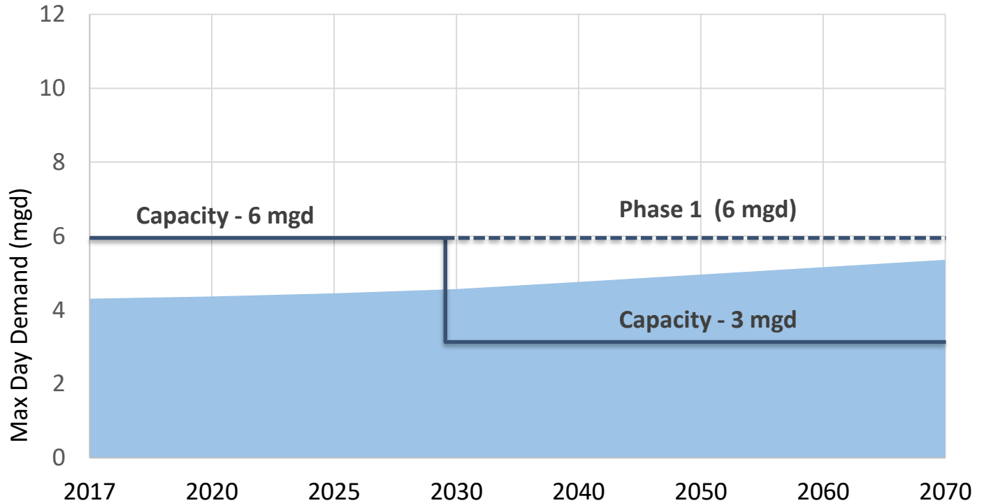
Chatham County N (w/Moncure) Water Demand vs. Capacity (Max Day)
